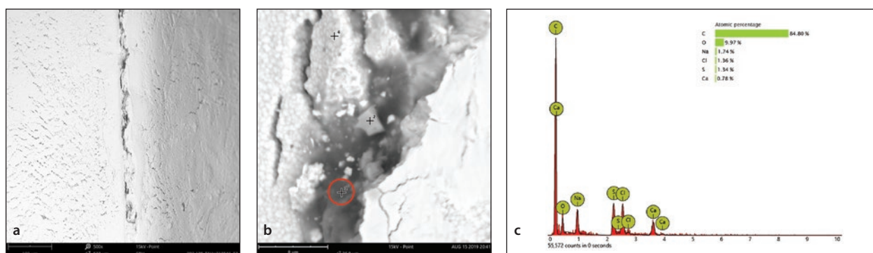
Fig 6 SEM/EDS analysis of the W Implant (TAV Dental). (a) SEM 500x, (b) SEM 10,000x with systematic organic contamination in a long material crack (> 500 \mu\text{m} ) on the implant shoulder, (c) differential EDS spot measurement (#1 minus #4). This organic impurity revealed mainly carbon and small amounts of oxygen, sodium, chlorine, sulfur, and calcium in the elemental analysis. (The embedded grey particle #2 showed signals of aluminum oxide.)
