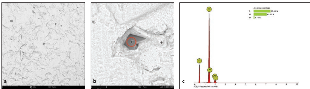
Fig 14 SEM/EDS analysis of the BioWin!/Standard Zirkon Implantat (Champions-Implants/ZV3). (a) SEM 500 \times , (b) SEM 5,000 \times with marked spots for EDS analysis; (c) differential EDS spot measurement of a single particle (5 to 10 \mu m) showed signals of aluminum and oxygen.
