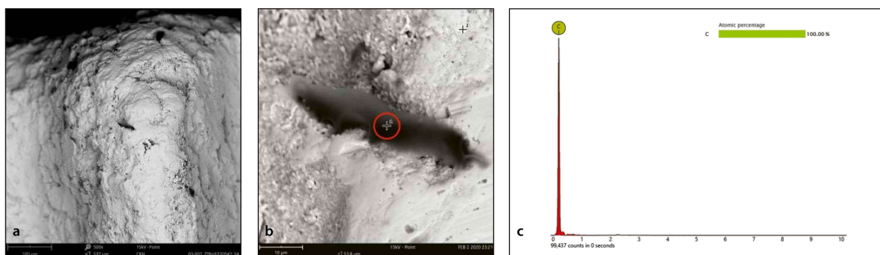
Fig 4 SEM/EDS analysis of the Zibone Implant (COHO Biomedical Technology). (a) SEM 500x, (b) SEM 5,000x with marked spots for EDS analysis, (c) differential EDS spot measurement (#1 minus #2); quantitative and qualitative elemental analysis revealed organic nature of the particle.
