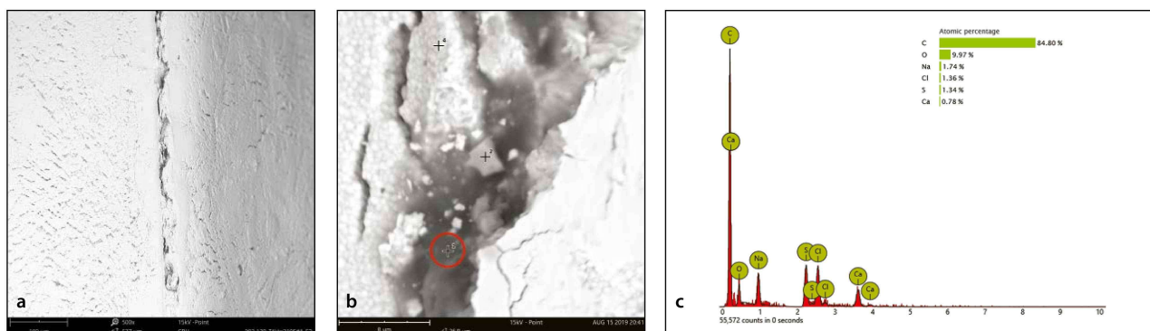
Fig 6 SEM/EDS analysis of the W Implant (TAV Dental). (a) SEM 500x, (b) SEM 10,000x with systematic organic contamination in a long material crack (> 500 \mu m) on the implant shoulder, (c) differential EDS spot measurement (#1 minus #4). This organic impurity revealed mainly carbon and small amounts of oxygen, sodium, chlorine, sulfur, and calcium in the elemental analysis. (The embedded grey particle #2 showed signals of aluminum oxide.)
