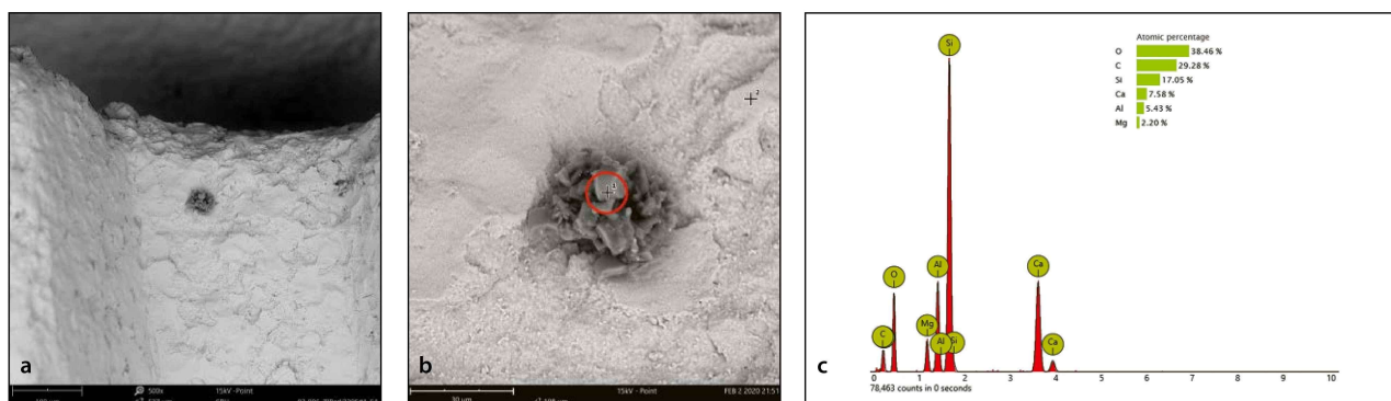
Fig 5 SEM/EDS analysis of the Zibone Implant (COHO Biomedical Technology). (a) SEM 500x, (b) SEM 2,500x with marked spots for EDS analysis, (c) differential EDS spot measurement (#1 minus #2); quantitative and qualitative elemental analysis showed different elements of the compound.
